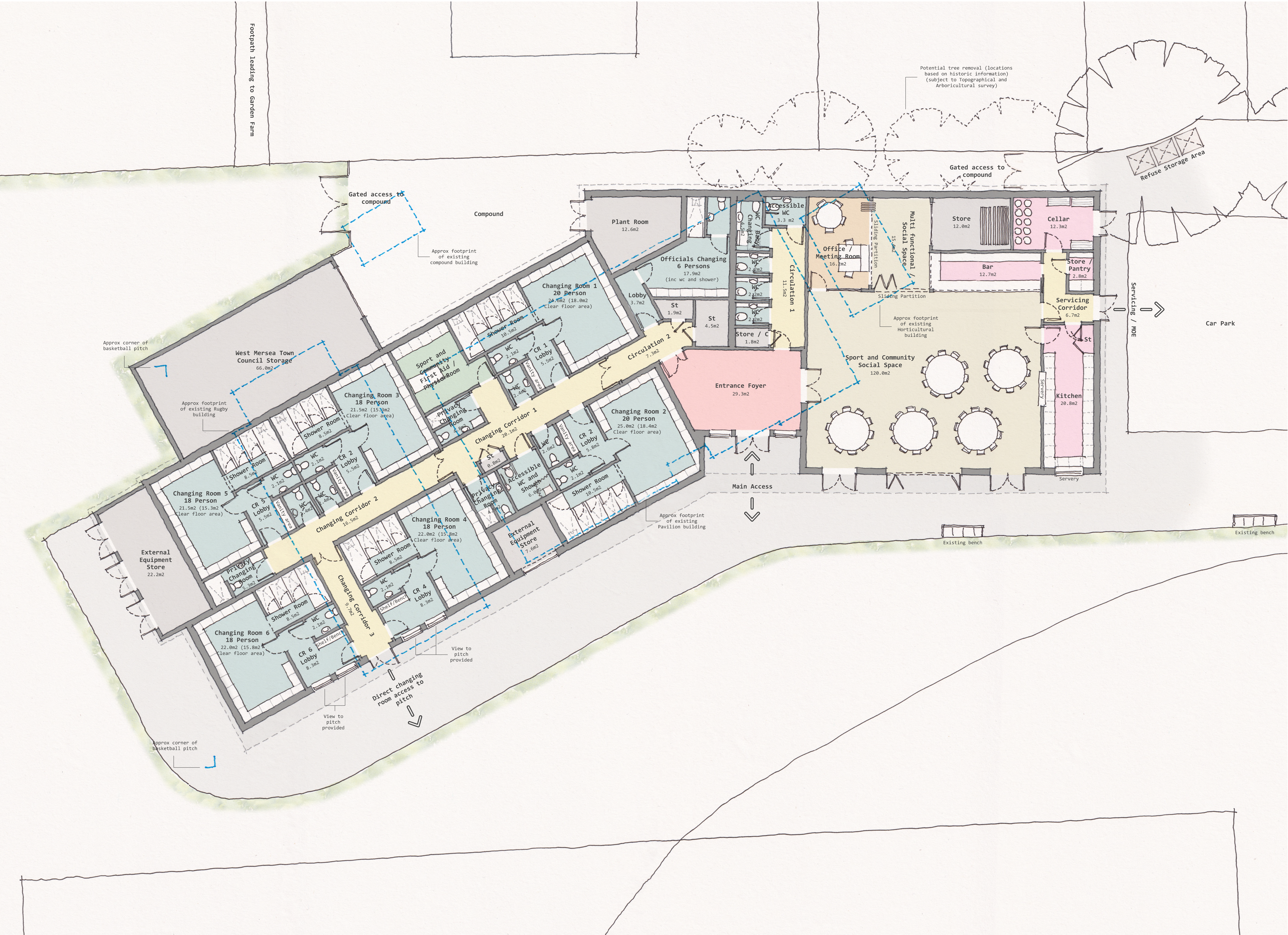
Proposed Ground Floor Plan (scale 1:100 @ A1)
